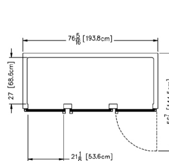
Plan - Three-Section
