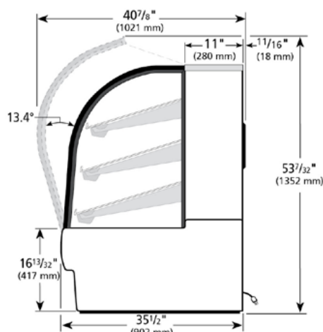
RIGHT VIEW
