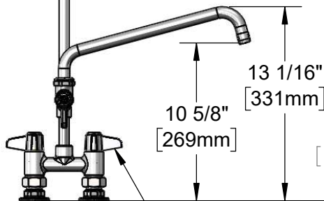
Quarter-Turn Ceramic Cartridges & equip Lever Handles w/ Color Coded Screws
