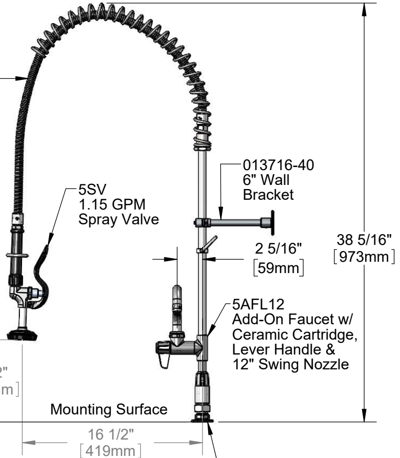
Ø 2" [51mm] Flanges w/ In-Line Check Valves & 1/2" NPT Female Inlets
