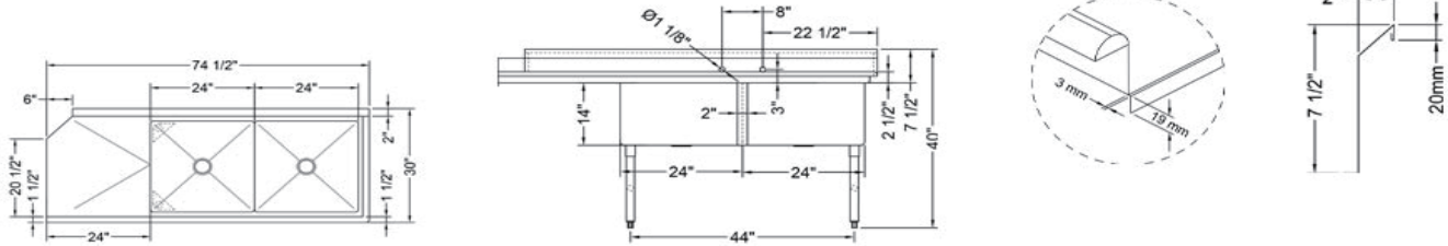
SI824-2R-DW DIMENSIONS
