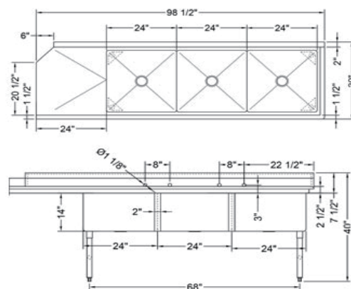
SI824-3R-DW DIMENSIONS
