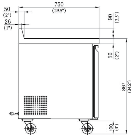
SECTION VIEW
