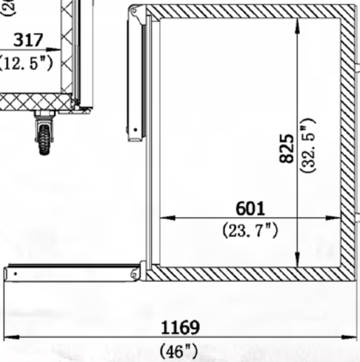
PRODUCT DRAWINGS
