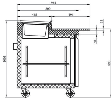
SECTION VIEW
