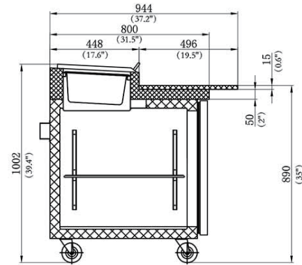
SECTION VIEW
