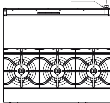
TOP VIEW 3/4" NPT GAS INLET 1 11/16"
