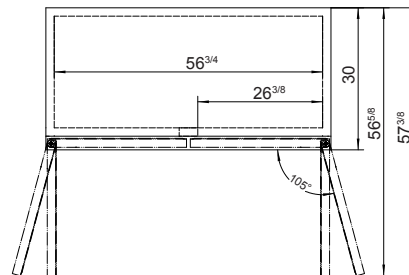
Rear grate
