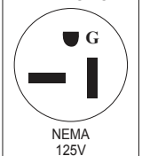
NEMA 5-20P
