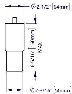
LEG DETAIL
