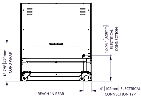
REACH-IN REAR
