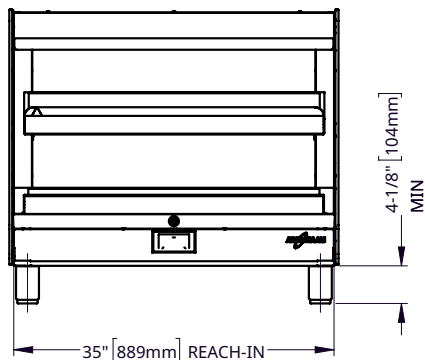
REACH-IN FRONT
