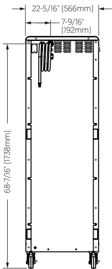
Shown with Simple control and 3-1/2" casters
